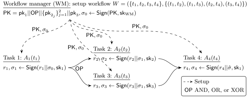
Fig. 2. Pattern for statically assigned workflows. The tuples (r_i, \sigma_i) denote the task reports corresponding to A_i(t_i) . If OP = \text{AND} then \hat{\sigma} \leftarrow \sigma_2 || \sigma_3 , if OP = \text{OR} then \hat{\sigma} \leftarrow \sigma_2, \hat{\sigma} \leftarrow \sigma_3 , or \hat{\sigma} \leftarrow \sigma_2 || \sigma_3 , if OP = \text{XOR} then \hat{\sigma} \leftarrow \sigma_2 or \hat{\sigma} \leftarrow \sigma_3 .
